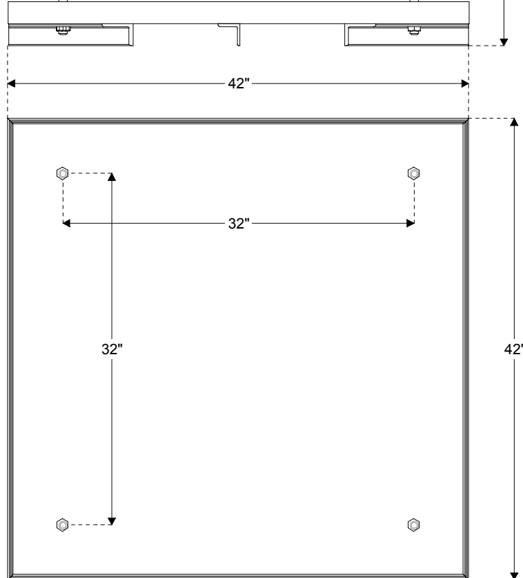
Support Base
